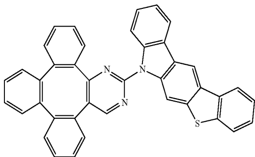
Compound 71
