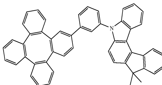
Compound 68
