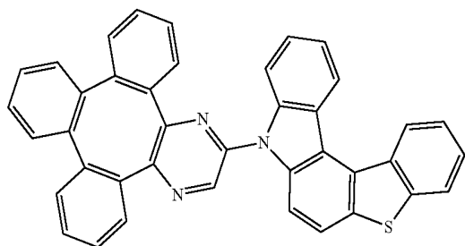
Compound 83
