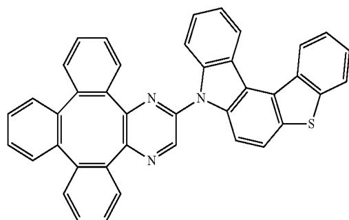
Compound 55
