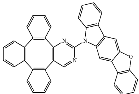
Compound 75
