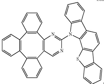
Compound 73
