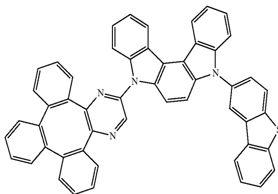
Compound 51
