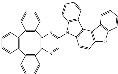
Compound 88
