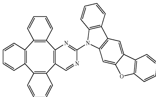
Compound 76
