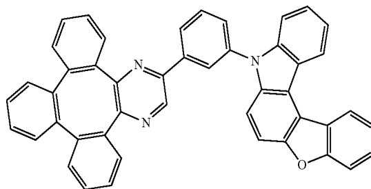
Compound 94
