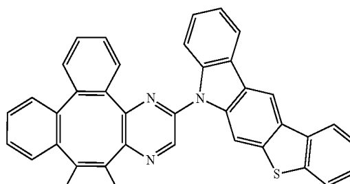
Compound 85
