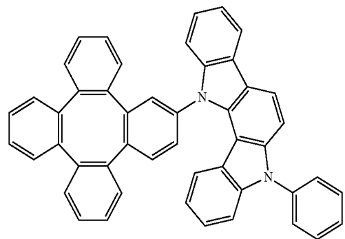
Compound 4
