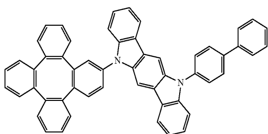
Compound 8
