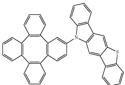
Compound 57
