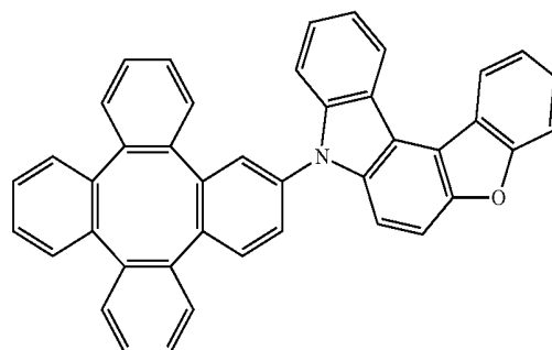
Compound 60
