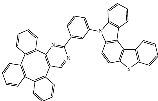
Compound 80
