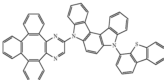
Compound 50
