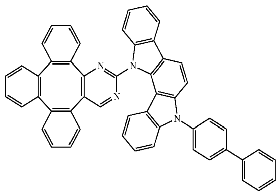
Compound 29
