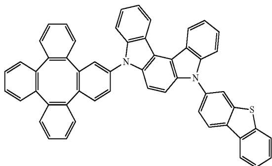
Compound 13
