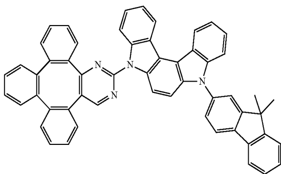
Compound 30
