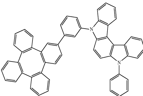
Compound 16
