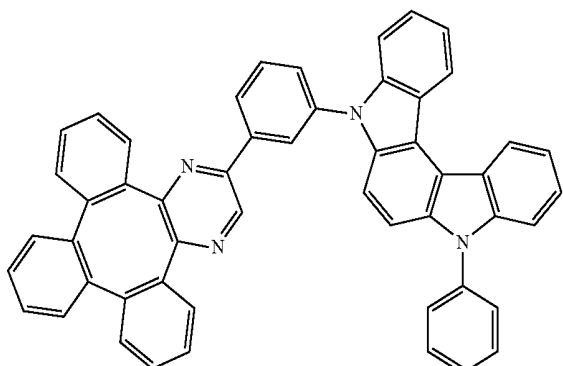
Compound 53
