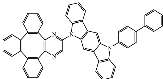
Compound 45
