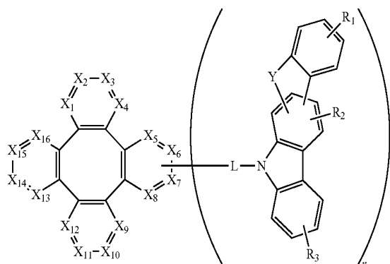
Formula 1
