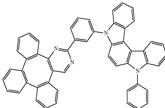
Compound 35
