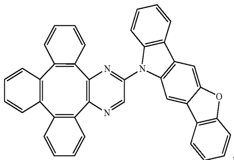
Compound 89
