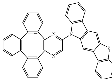
Compound 85
