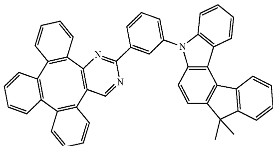
Compound 83
