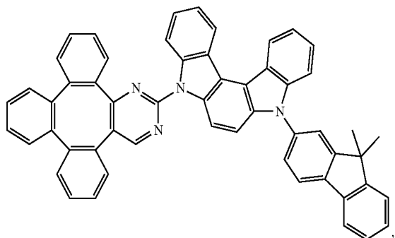
Compound 30
