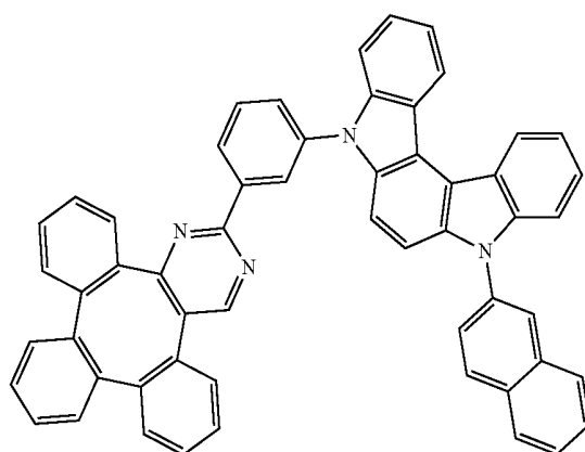
Compound 37
