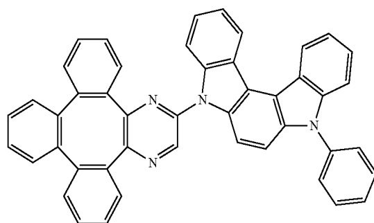
Compound 37
