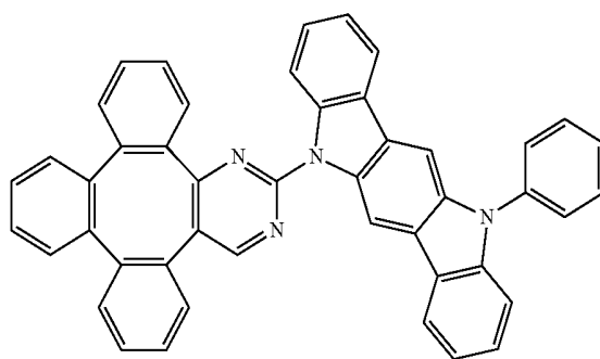
Compound 20
