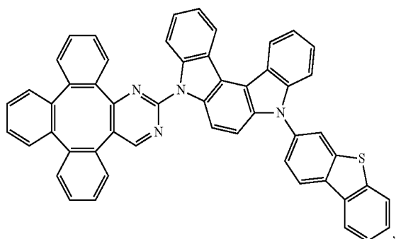
Compound 31
