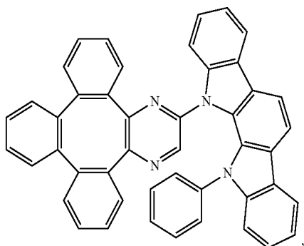
Compound 41
