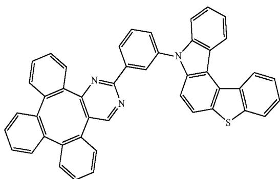
Compound 81
