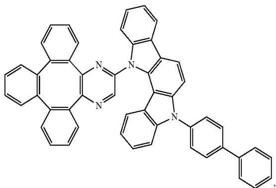
Compound 46
