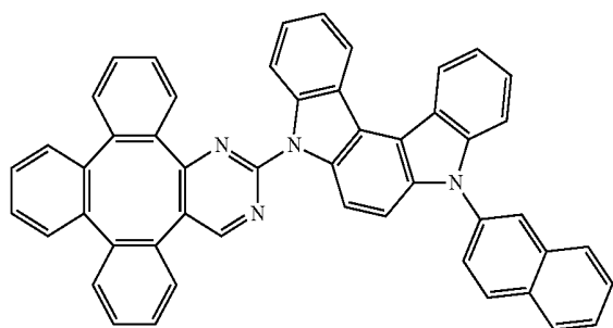
Compound 24
