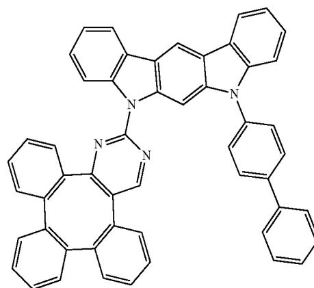
Compound 28
