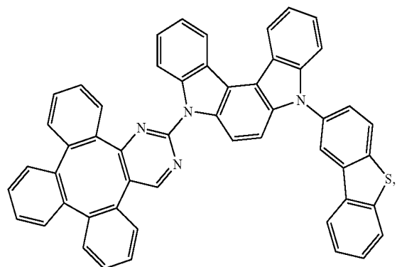
Compound 33
