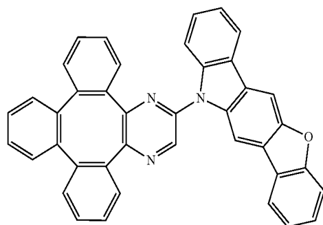
Compound 89
