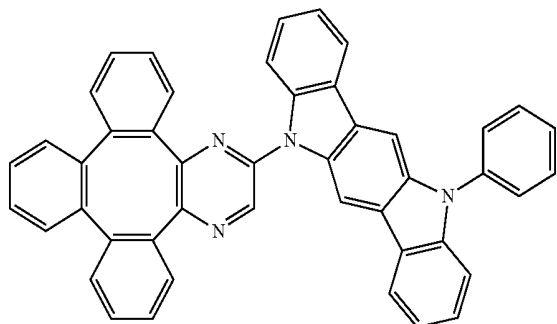
Compound 38
