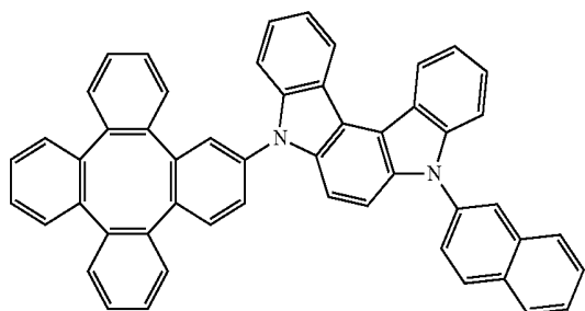
Compound 6
