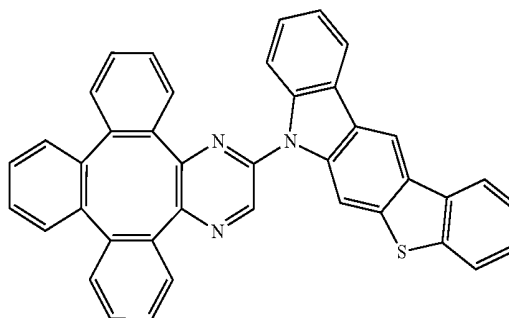
Compound 85
