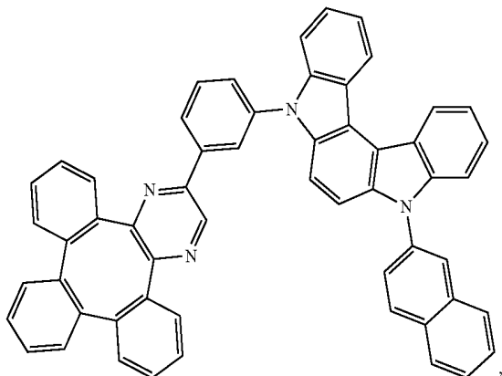
Compound 54
