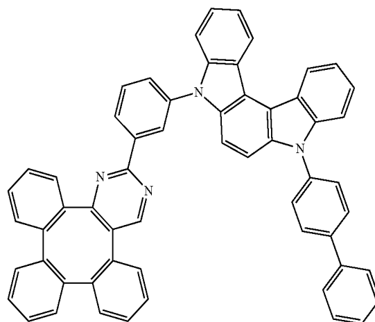
Compound 35
