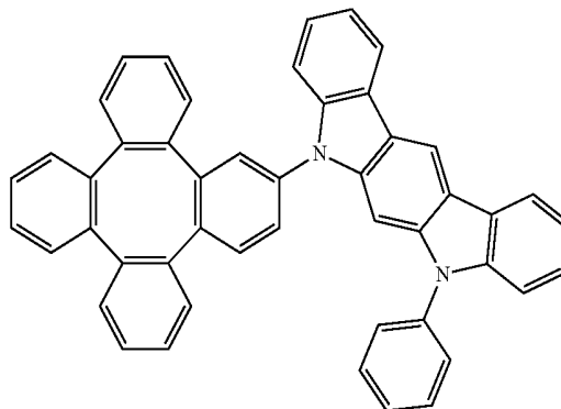
Compound 3
