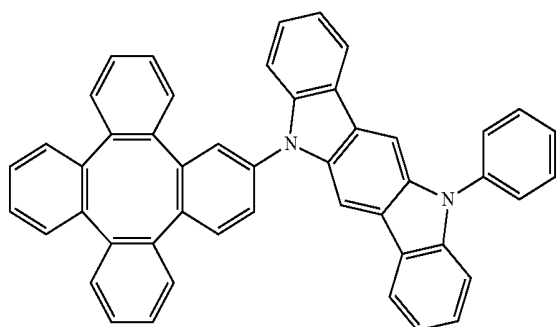
Compound 2
