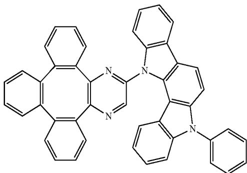
Compound 41
