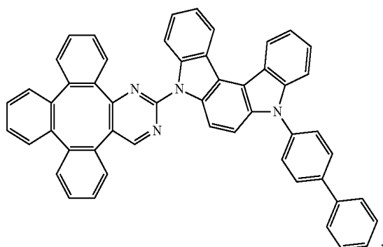
Compound 25
