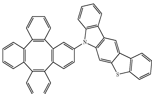
Compound 57
