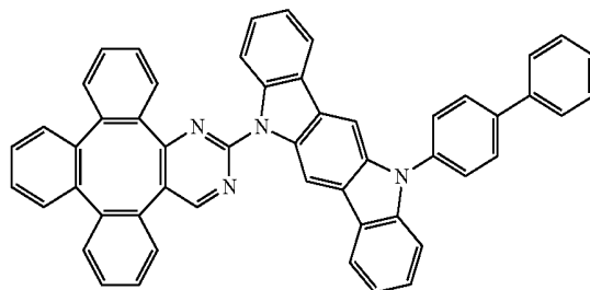
Compound 26
