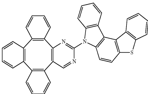
Compound 69
