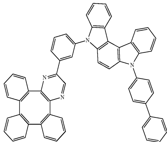
Compound 53
