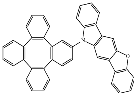
Compound 61
