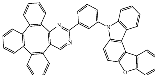
Compound 82
