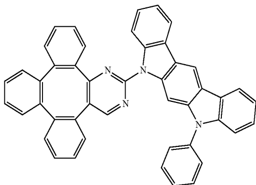
Compound 21
