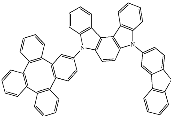
Compound 15
