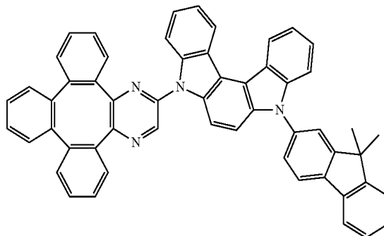
Compound 48
