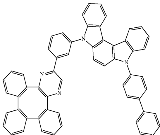
Compound 54
