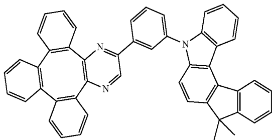
Compound 95
