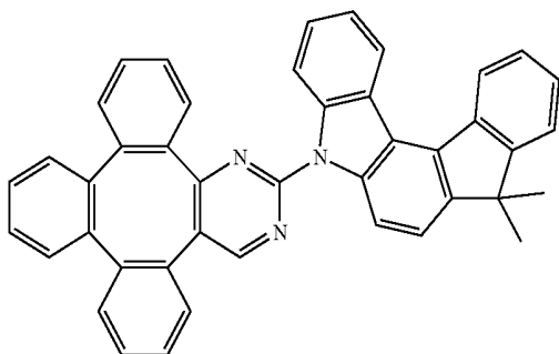
Compound 80
