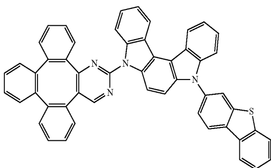
Compound 31
