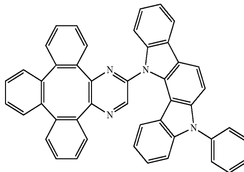
Compound 40
