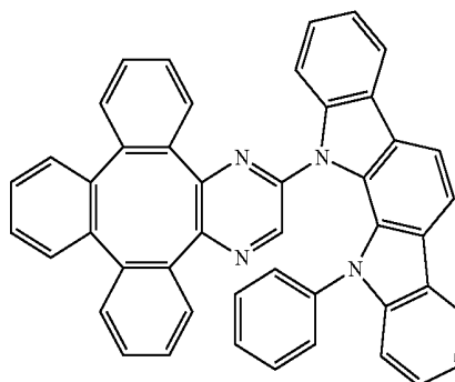
Compound 37
