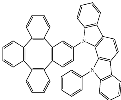
Compound 1
