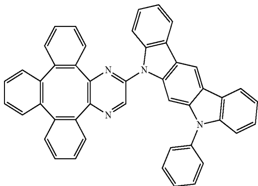
Compound 39
