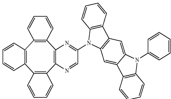
Compound 39
