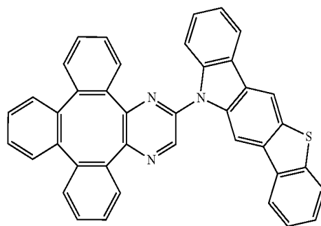
Compound 84
