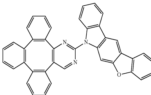
Compound 76
