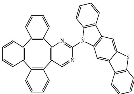
Compound 70
