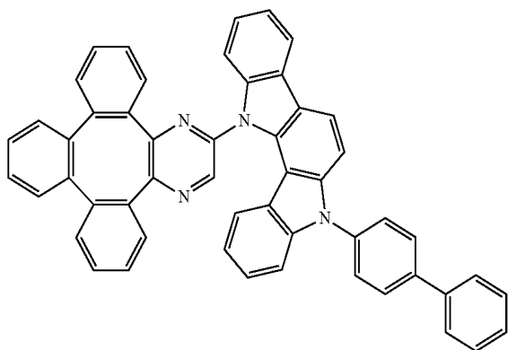
Compound 47
