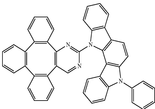
Compound 22
