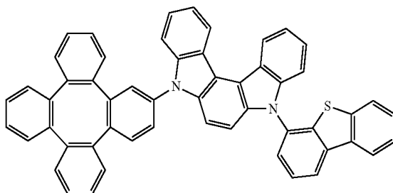
Compound 14
