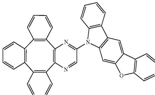
Compound 91
