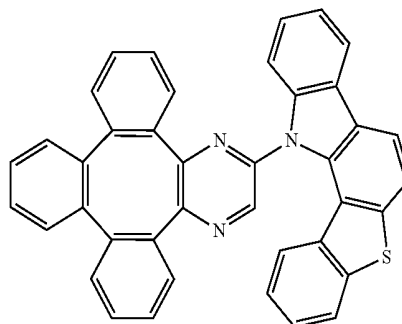
Compound 82
