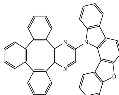
Compound 87
