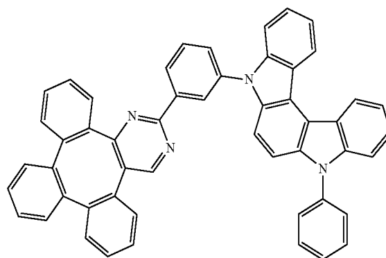
Compound 34
