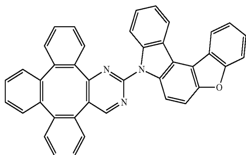
Compound 74
