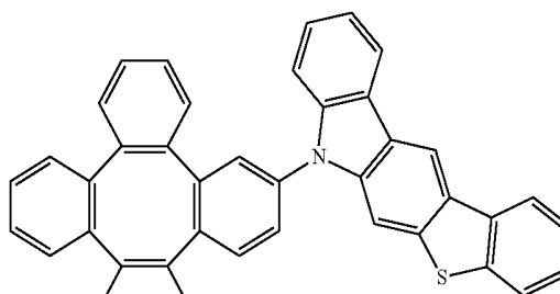
Compound 57
