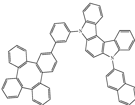
Compound 19
