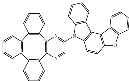
Compound 88
