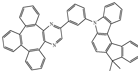
Compound 95
