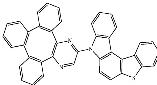
Compound 84
