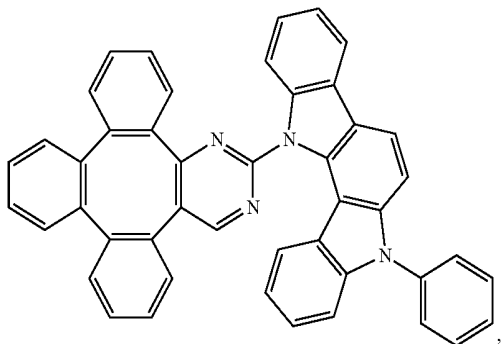
Compound 22
