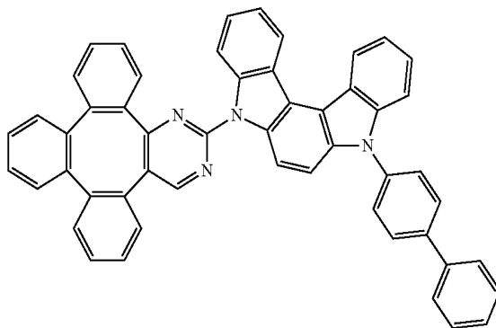
Compound 25
