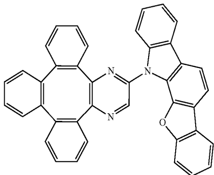
Compound 92
