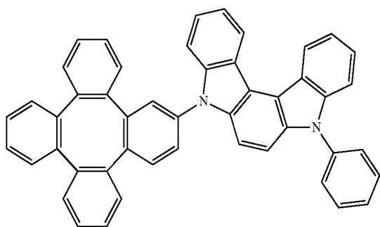
Compound 1
