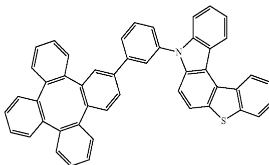
Compound 67
