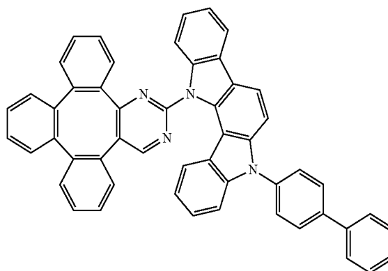
Compound 28
