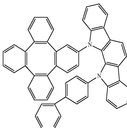
Compound 7
