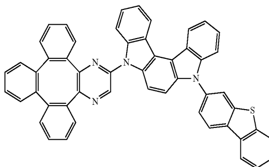
Compound 49
