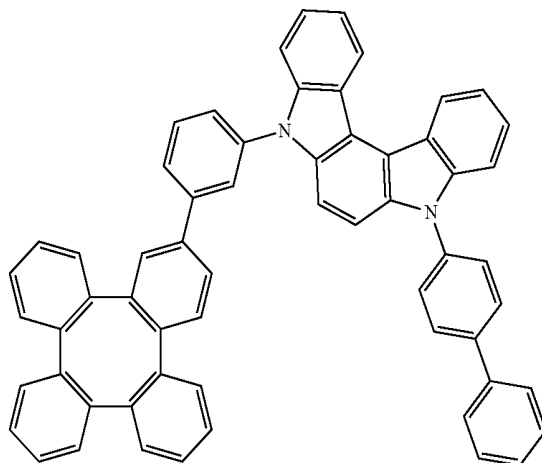
Compound 18
