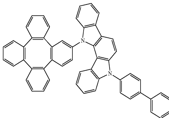
Compound 11
