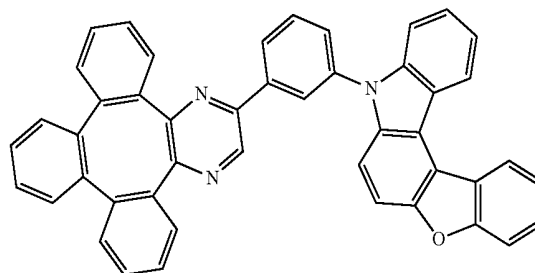
Compound 94
