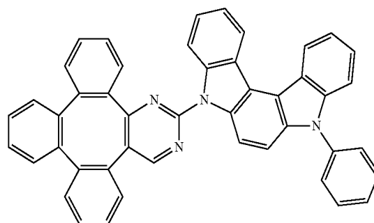
Compound 20
