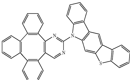
Compound 71
