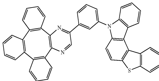
Compound 93
