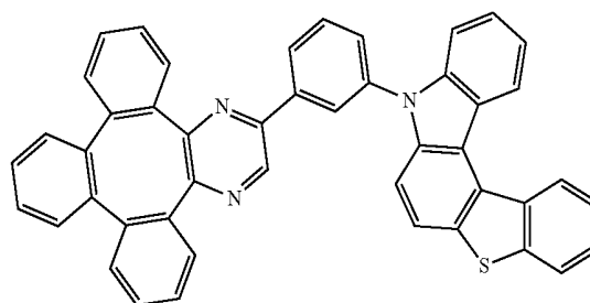
Compound 94
