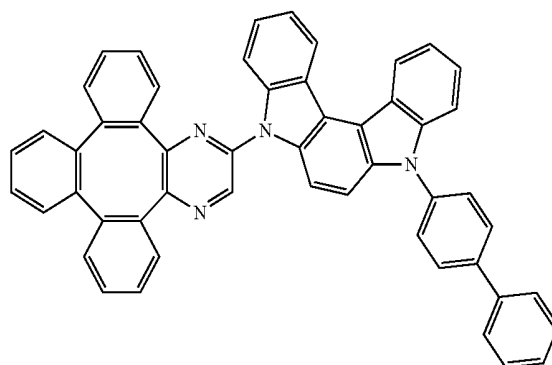
Compound 43
