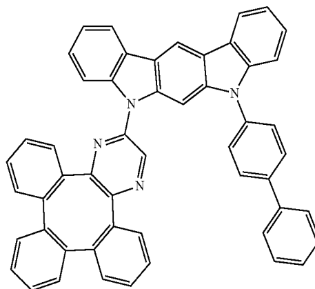
Compound 45
