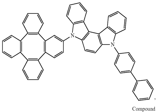
Compound 7
