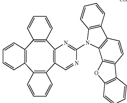
Compound 78
