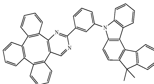
Compound 83
