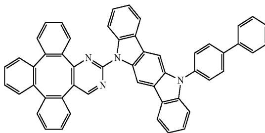
Compound 26
