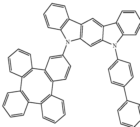
Compound 10
