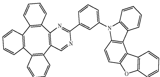
Compound 82
