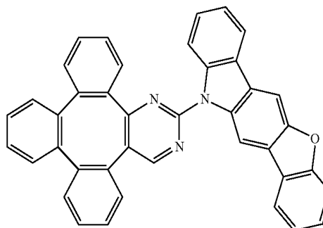
Compound 75
