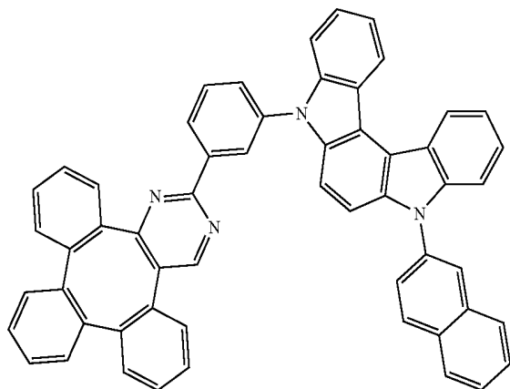
Compound 36
