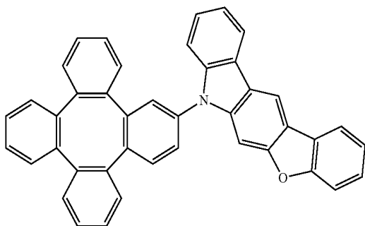
Compound 62
