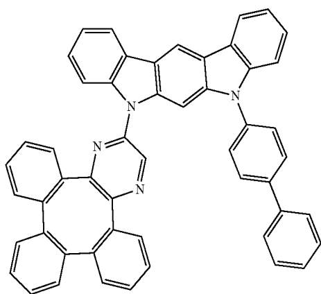
Compound 45
