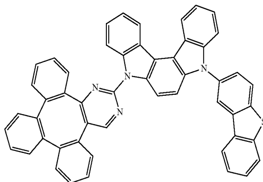
Compound 33
